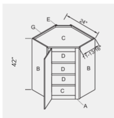
42"High Diagonal Corner Wall Cabinet
