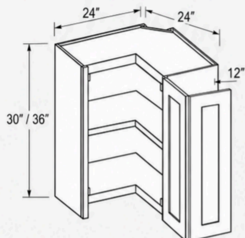
30" / 36" High Easy-Reach Corner Wall Cabinet
