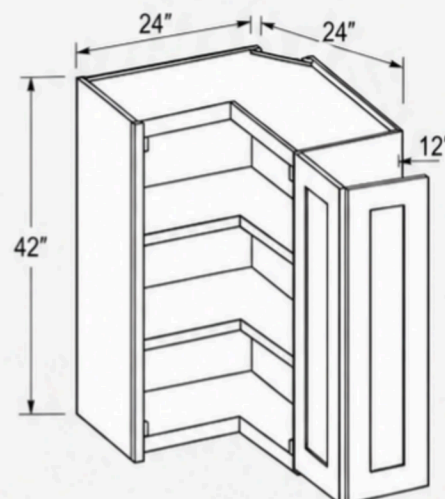
42" High Easy-Reach Corner Wall Cabinet
