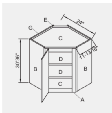
30"High 36"High Diagonal Corner Wall Cabinet
